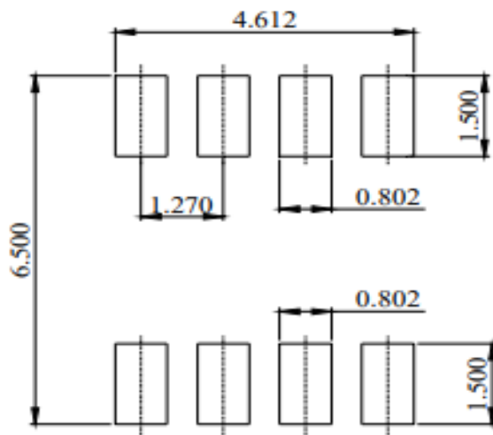
DIMENSIONS: MILLIMETERS
